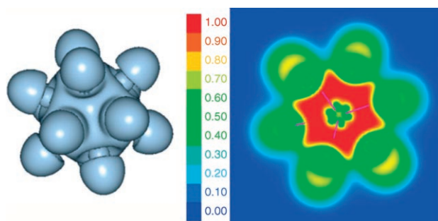
Figure 4. Isosurface (left) and cut-plane (right) ELF representations for \text{Pu@Pb}_{12} .
